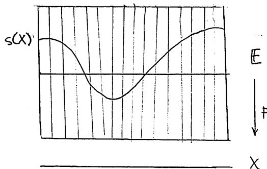
FIGURE 6. Section of a vector bundle
