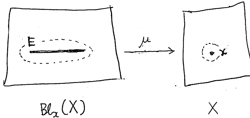
FIGURE 7. Blowing up a point x \in X .
