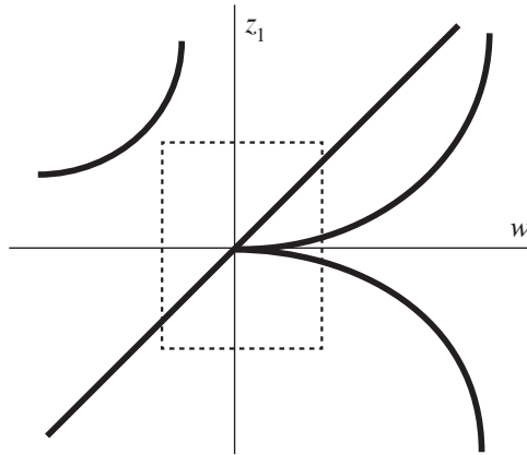
FIGURE 1. Zeroes of a function with Weierstrass polynomial p = (z_1 - w)(z_1^2 - w^3) .
