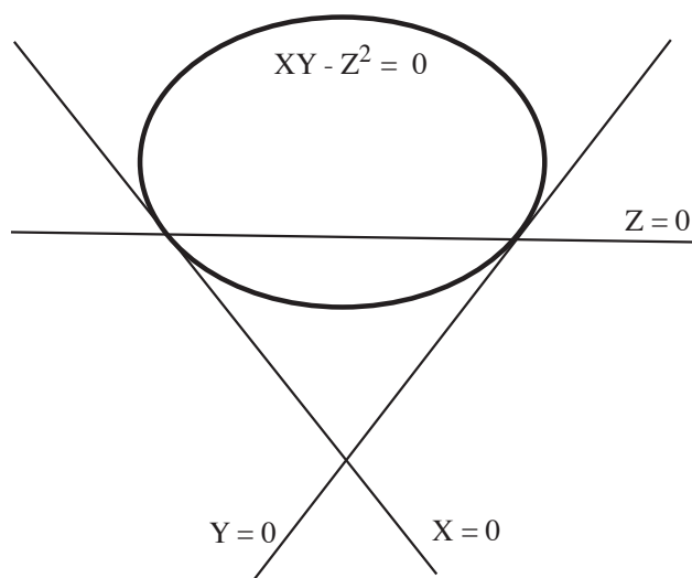
FIGURE 2. The conic XY = Z^2 in \mathbf{P}^2 .
