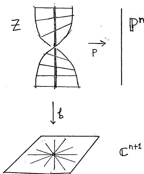
FIGURE 3. Blowing up the origin in \mathbf{C}^{n+1}
