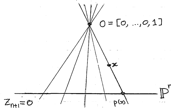
FIGURE 5. The hyperplane line bundle
